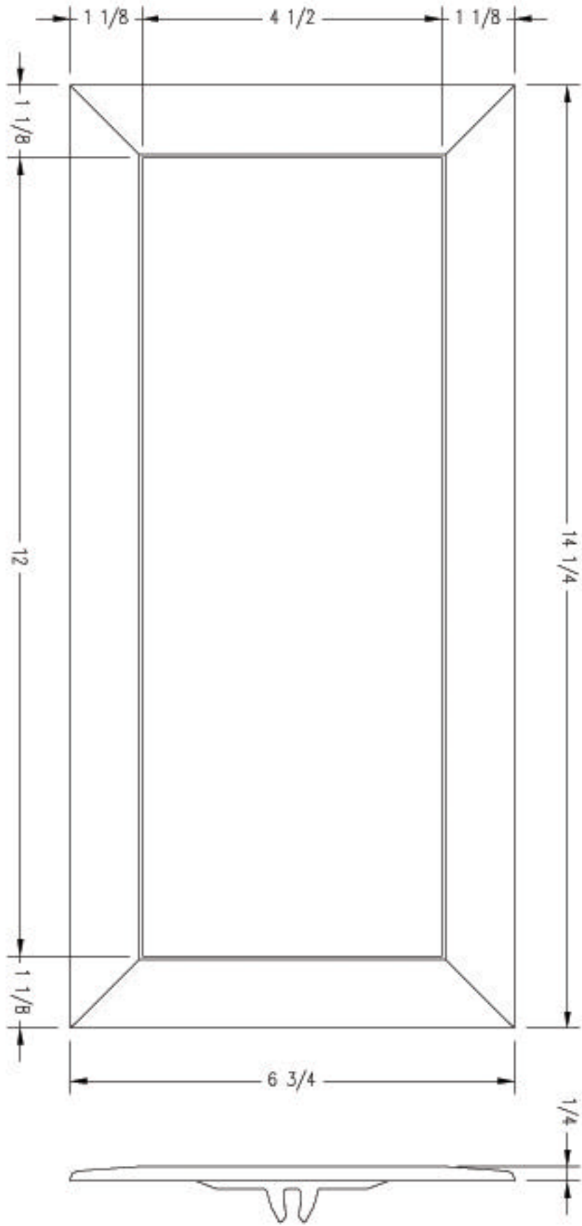
FRONT VIEW
