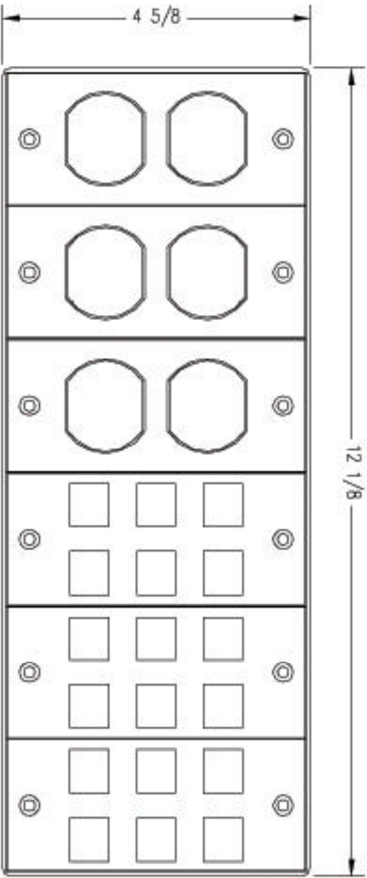
TOP VIEW
